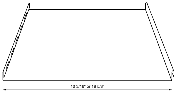
Panel Profile
