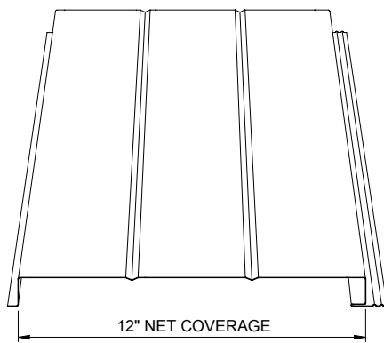
PANEL PROFILE
