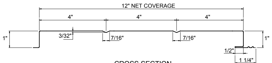
CROSS SECTION (NON-STRUCTURAL PANEL)
